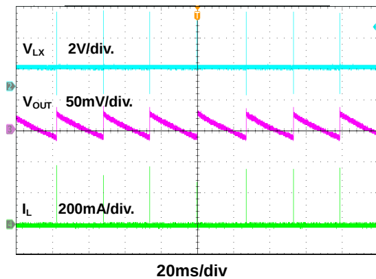
Figure 16. Steady State Waveform
