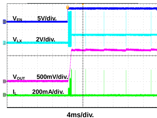
Figure 12. Power On Through EN Waveform
