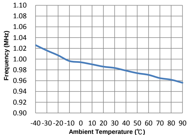
Figure 7. Frequency vs. Ambient Temperature
