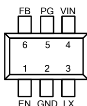
Figure 1. Pin Assignment of FP6397
