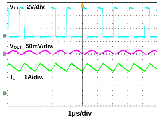
Figure 17. Steady State Waveform
