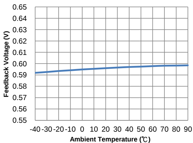
Figure 6. Feedback Voltage vs. Ambient Temperature
