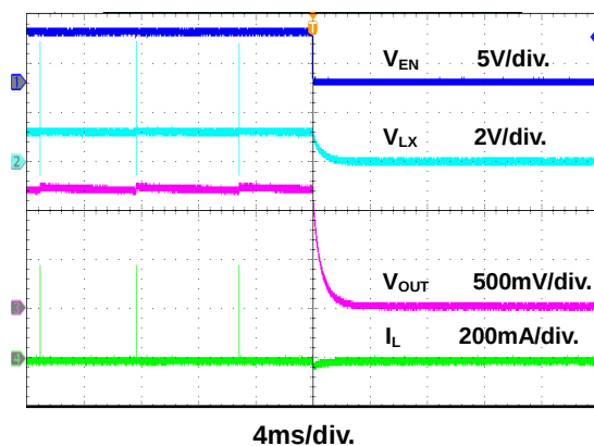
Figure 14. Power Off Through EN Waveform
