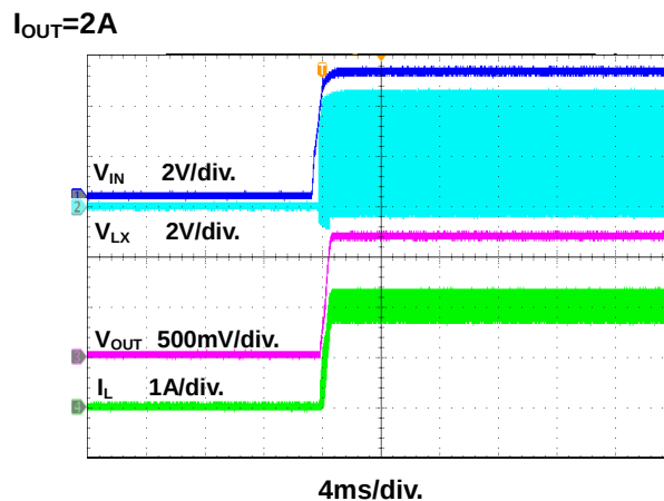
Figure 9. Power On Through VIN Waveform
