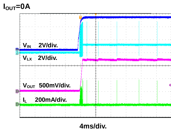
Figure 8. Power On Through VIN Waveform
