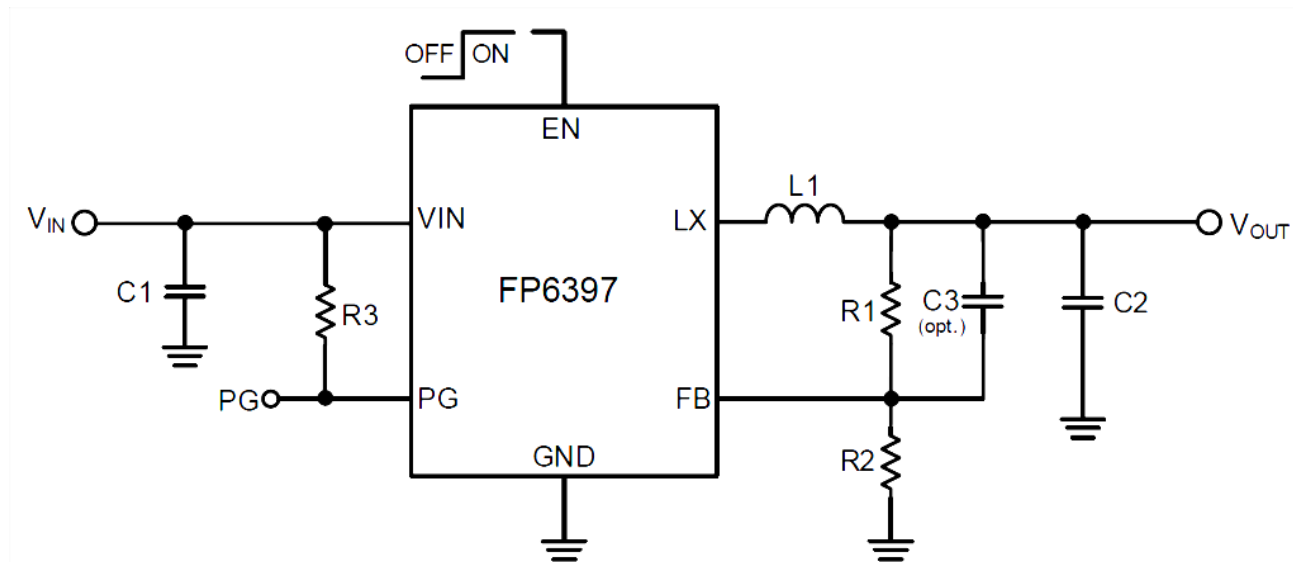
Figure 2. Schematic Diagram
