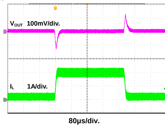
Figure 18. Load Transient Waveform
